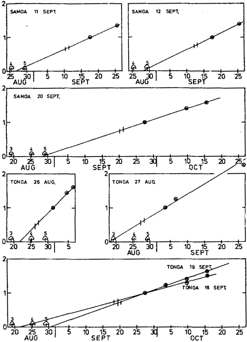
FIGURE 3. THE ORIGIN OF FRESH FISSION PRODUCTS IN AIR FILTER SAMPLES 1973 (concl.)
